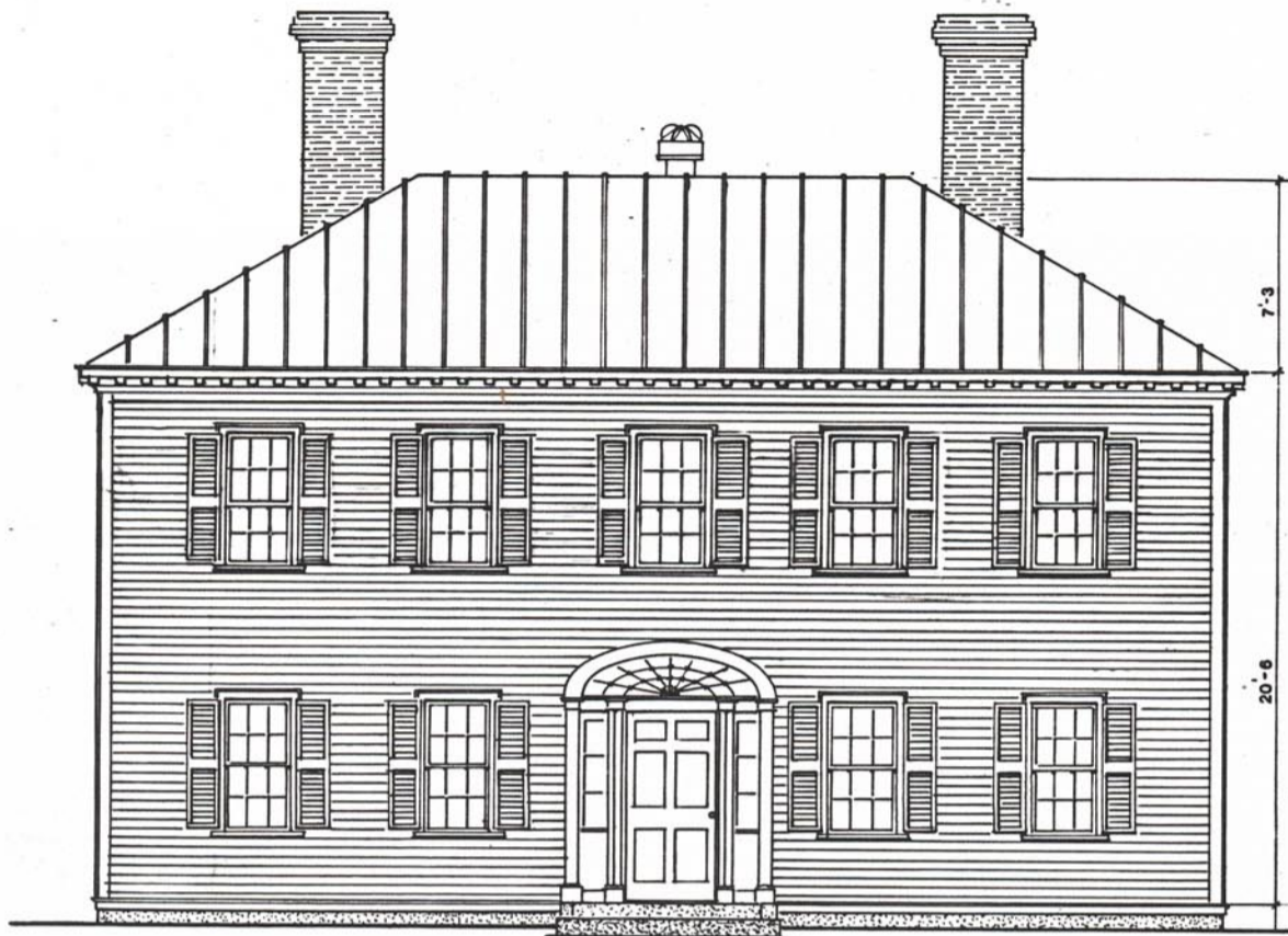
WEST ELEVATION
